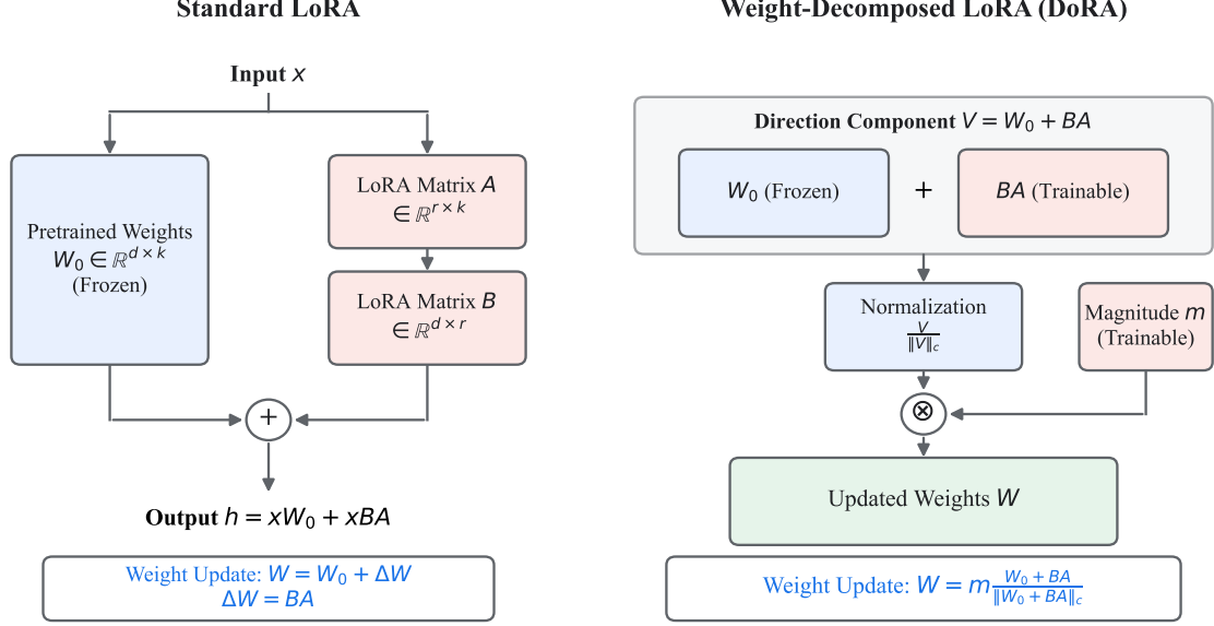
Figure 4.4: Architectural comparison between Standard LoRA (left) and Weight-Decomposed LoRA (DoRA, right). While LoRA directly adds the low-rank update to the pre-trained weights, DoRA decomposes the weights into magnitude ( m ) and directional components, applying the low-rank update strictly to the normalized direction before re-scaling by the trainable magnitude.
