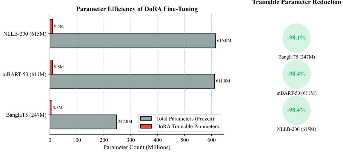
Figure 4.5: Parameter efficiency of DoRA fine-tuning across the three evaluated model architectures, demonstrating over 98% reduction in trainable parameters compared to full fine-tuning.
