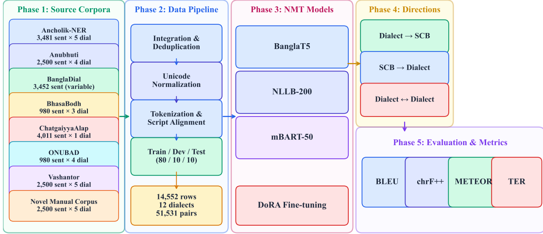
Figure 1.2: End-to-end architectural workflow of the Poly-Dialectal Neural Machine Translation Framework, depicting five phases: source corpora integration from seven existing datasets and one novel manual corpus, the data processing pipeline, NMT model fine-tuning with DoRA, multi-directional translation paradigm, and evaluation with four standard MT metrics.
