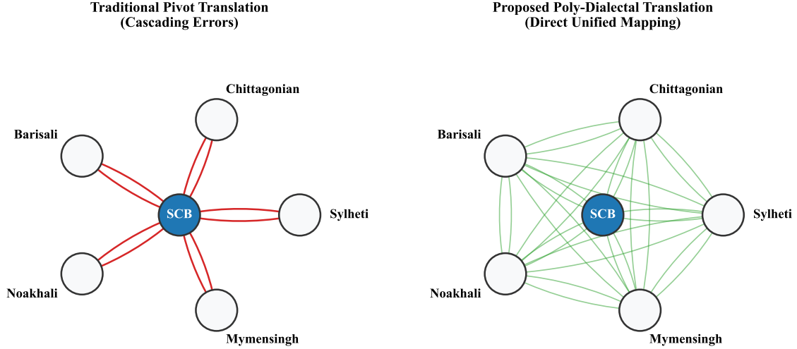
Figure 1.1: Structural comparison between the traditional pivot translation approach (routing through Standard Bangla) and the proposed direct poly-dialectal mapping topology.
